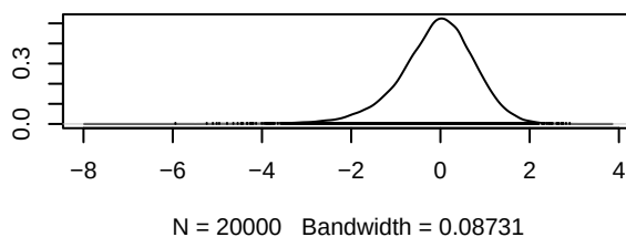
Density of d.chemo.Afatinib
